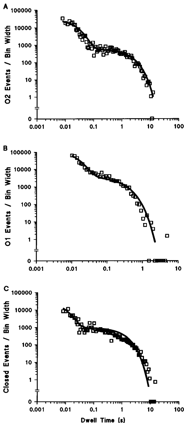
FIGURE 5 Demonstration of biexponential nature of channel states as measured at 37°C and +15 mV. (A) O2; (B) O1; (C) closed. Note that all states were clearly composed of more than one exponential component.
