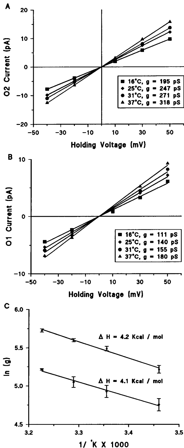
FIGURE 2 Temperature dependence of open channel conductance through (A) the O2 state and (B) the O1 state from an individual experiment. Note that the voltage dependence remained linear throughout the range of potentials employed. (C) The temperature dependence of the O2 (top trace) and O1 (bottom trace) displayed as an Arrhenius plot. The ratio of conductances remained constant and gave a calculated enthalpy for conduction of 4.2 kcal/mol for O2 and 4.1 kcal/mol for O1 (data plotted \pm SEM, n = 4 to 6).
